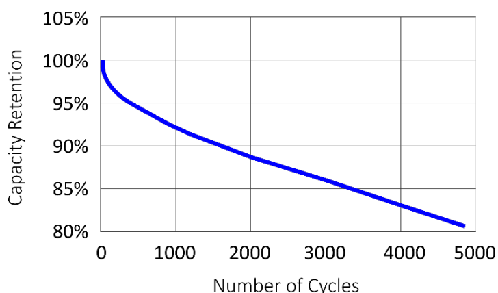
BATTERY CYCLE LIFE AT 25°C (1C/1C)
